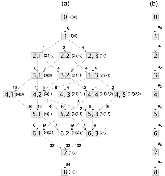
FIG. 2. Width diagrams for the breaking process of N=8 . (a) Primary diagram. The various configurations are labeled by the integers inside the boxes. The integers in parentheses at the right of the boxes represent the two N=4 configurations juxtaposed to form each of the N=8 configurations. The number accompanying an arrow connecting two boxes stands for the dimensionless partial decay width of that transition. (b) Effective diagram. This is obtained from (a), and is used to obtain rigorous bounds for the next height, N=16 . The a s are explained in the text.
