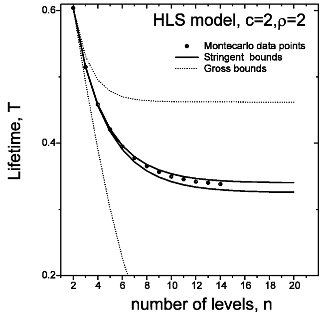
FIG. 4. Dimensionless lifetime, T , for a fractal tree of height n : the circles are obtained from Monte Carlo simulations; the continuous lines are the stringent bounds, and the dotted lines are the gross bounds.
