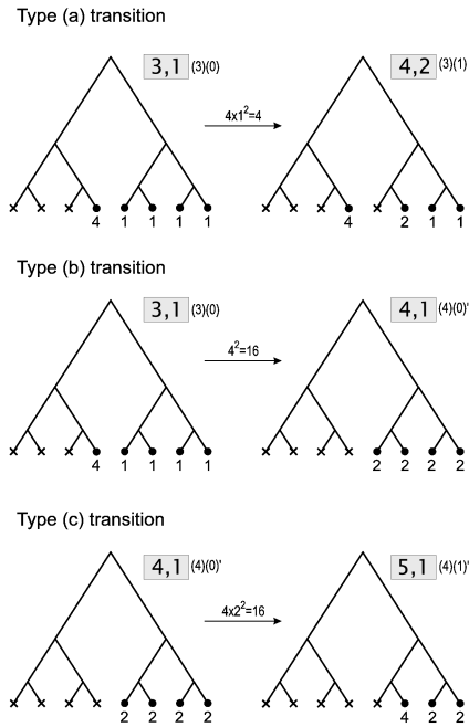
FIG. 3. Relation between the explicit and the symbolic notations for configurations of N=8 , built juxtaposing pairs of N=4 . See the text for details.
