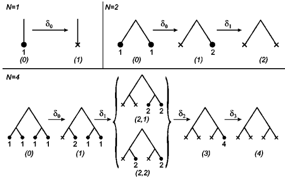
FIG. 1. Breaking process for the three smallest trees of coordination c=2 ( N=1,2,4 ). The integers in parentheses ( r ) represent the number of breakings that has occurred. The \delta s stand for the time steps elapsed between successive individual breakings and the numbers under the legs indicate the load they bear.
